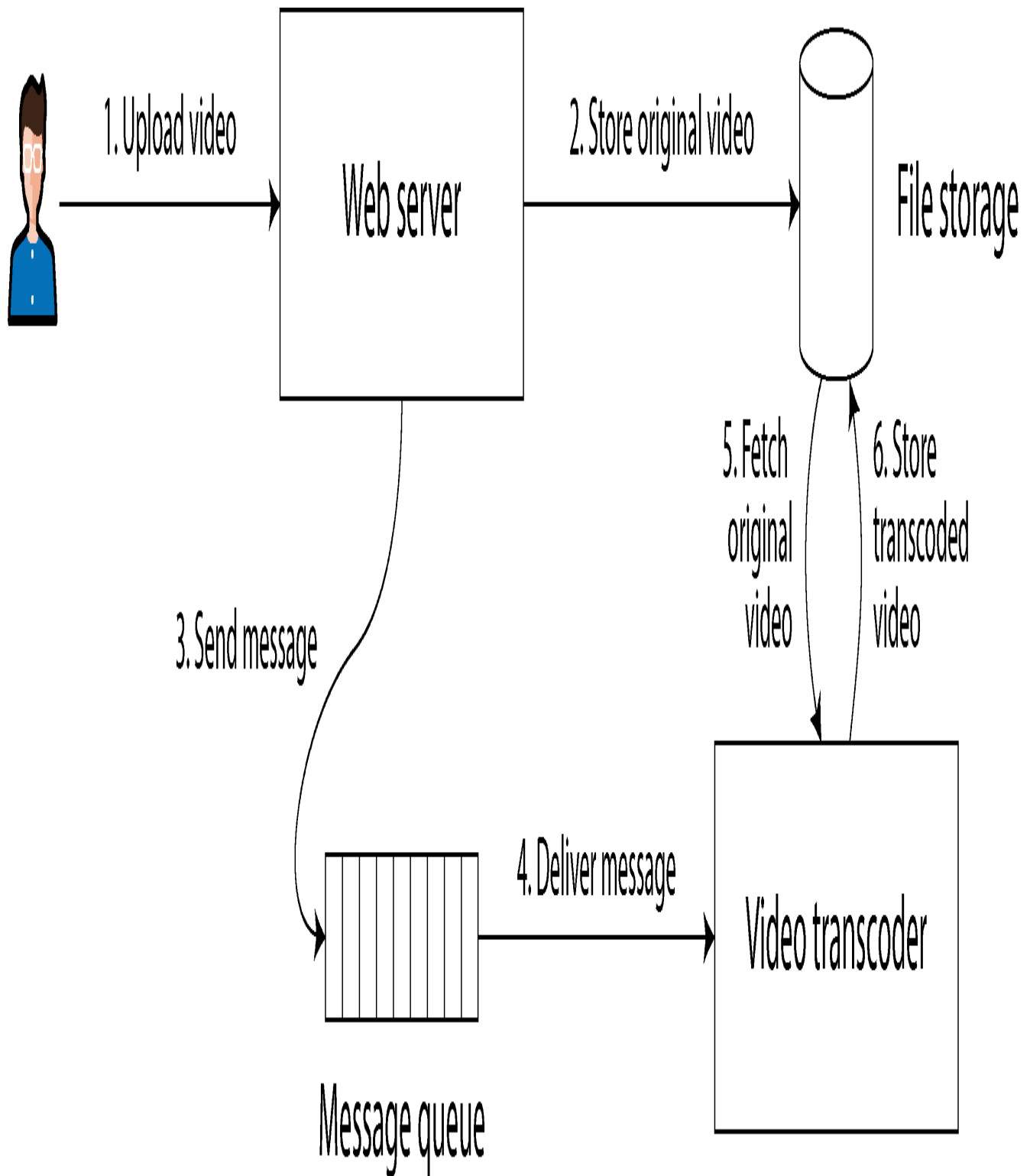
Figure 10-5. The web server and video transcoder communicate through both file storage and a message queue, opening the potential for race conditions.
