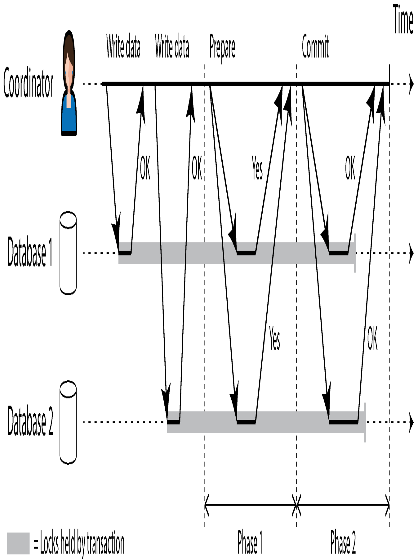
Figure 8-13. A successful execution of 2PC
