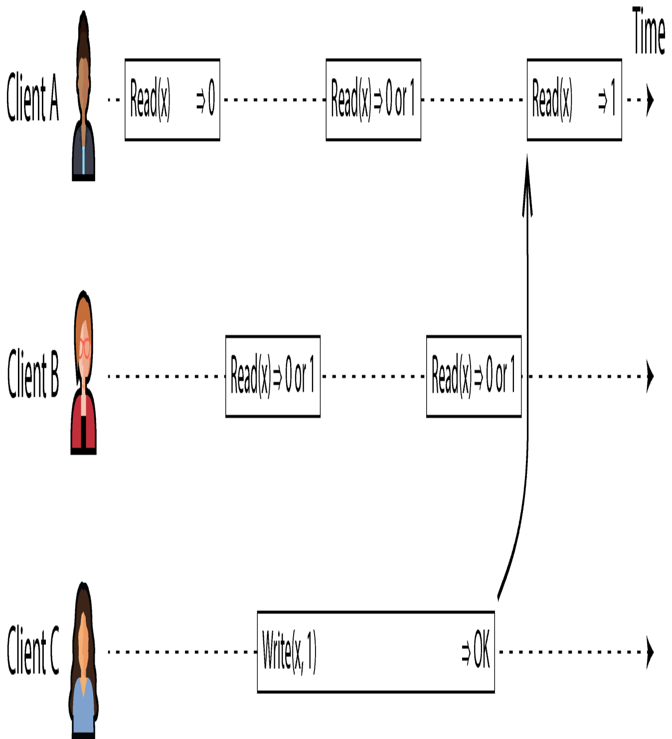
Figure 10-2. If a read request is concurrent with a write request, it may return either the old or the new value.
