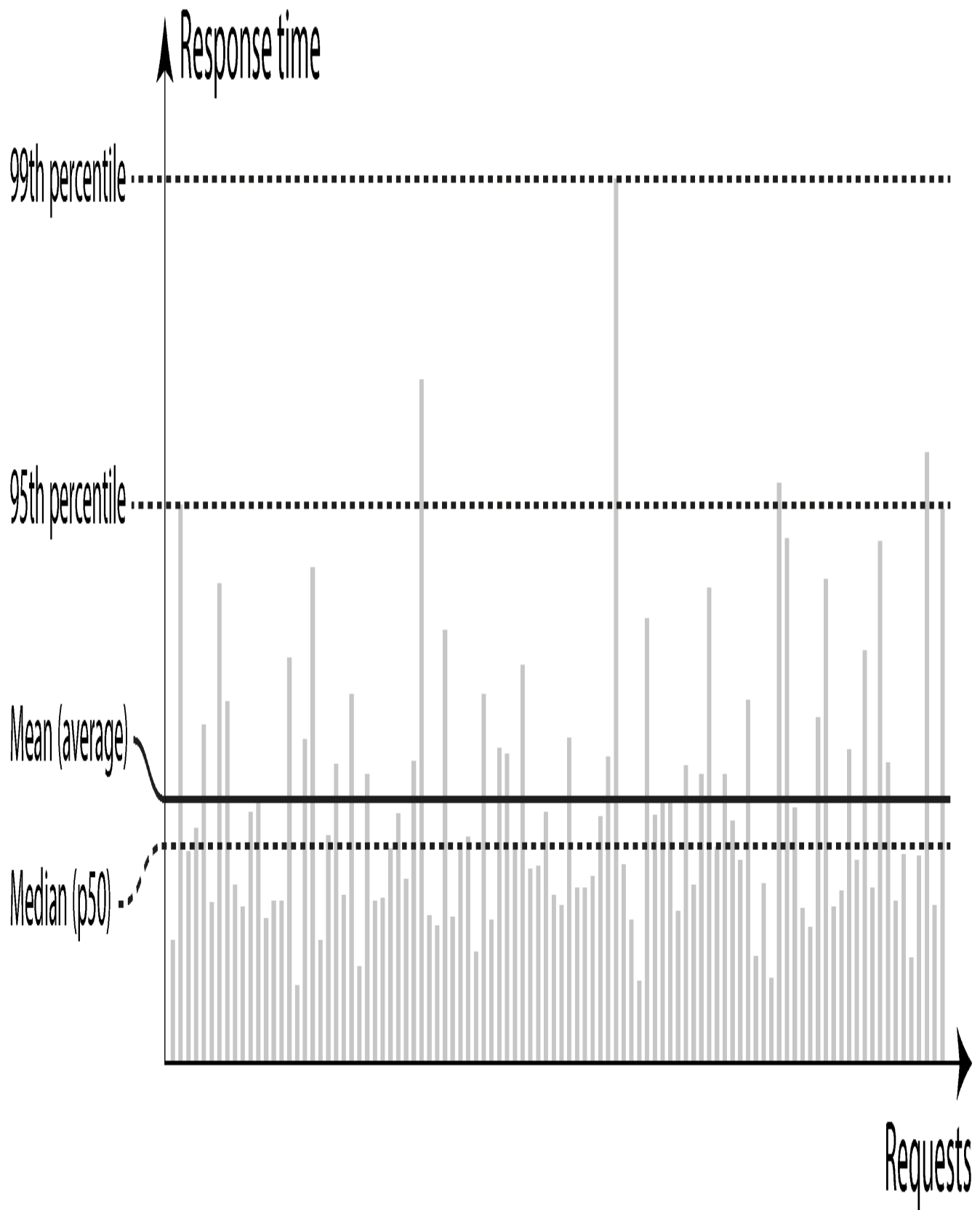
Figure 2-5. Illustrating mean and percentiles: response times for a sample of 100 requests to a service
