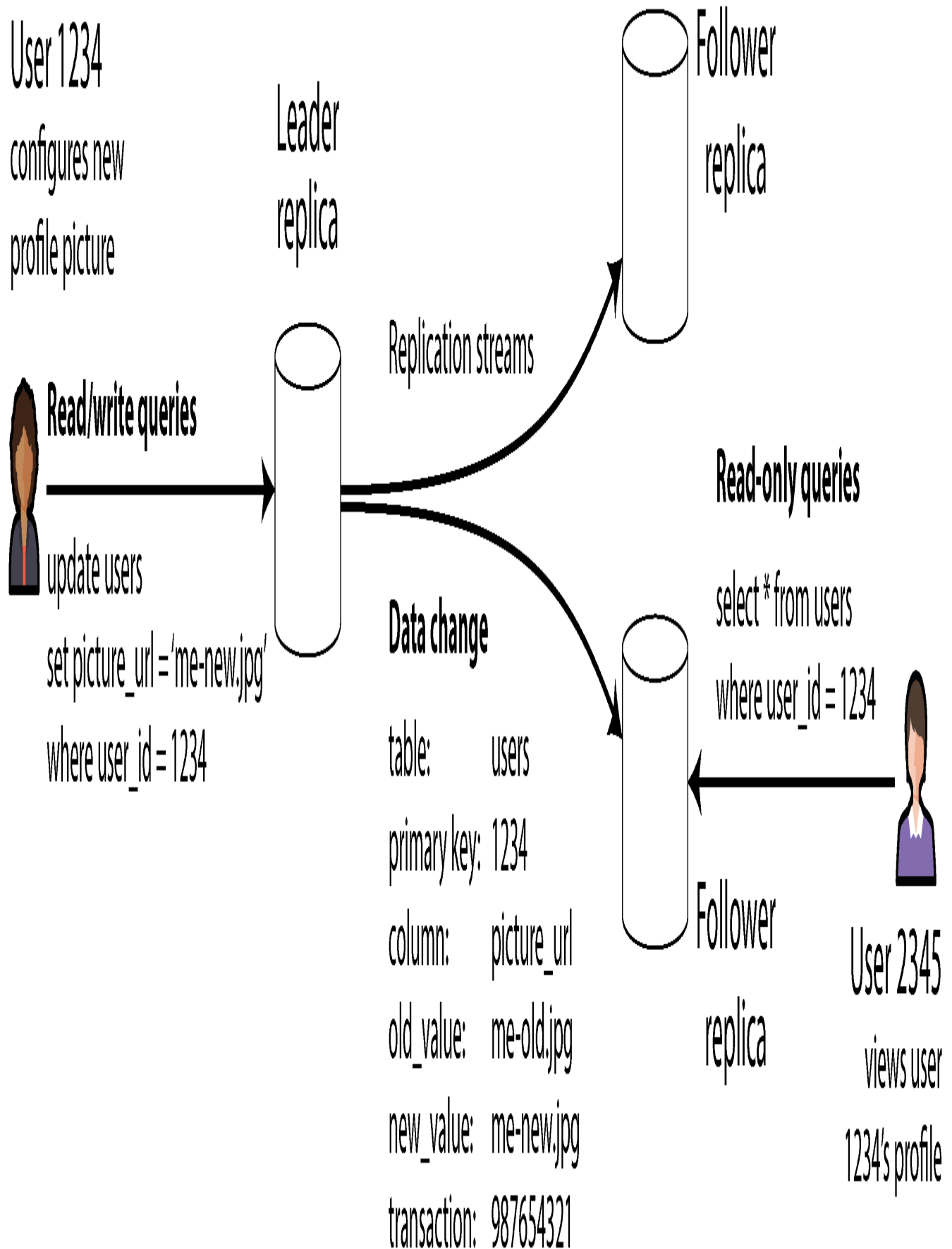
Figure 6-1. Single-leader replication directs all writes to a designated leader, which sends a stream of changes to the follower replicas.
