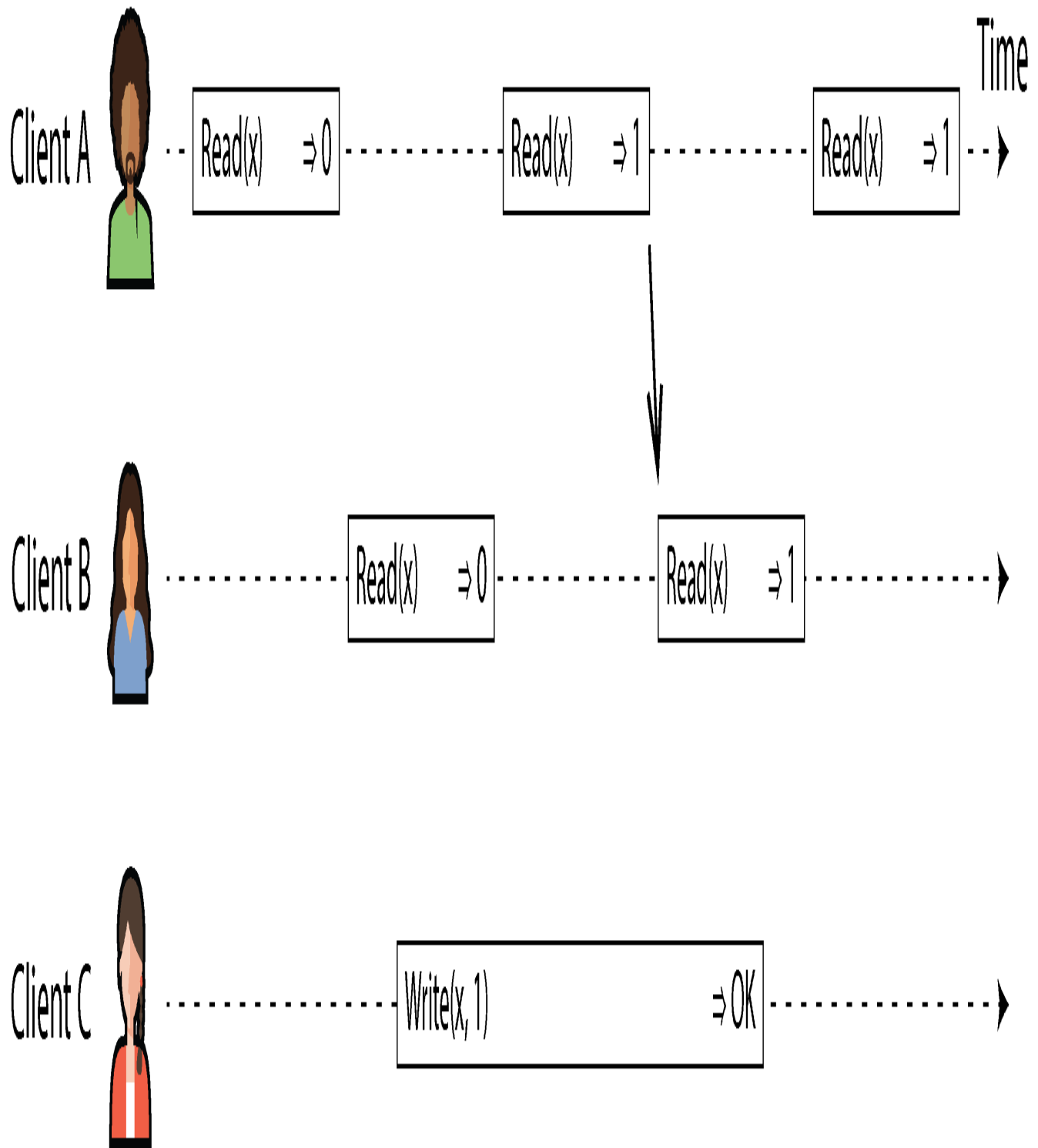
Figure 10-3. After any one read has returned the new value, all following reads (on the same or other clients) must also return the new value.
