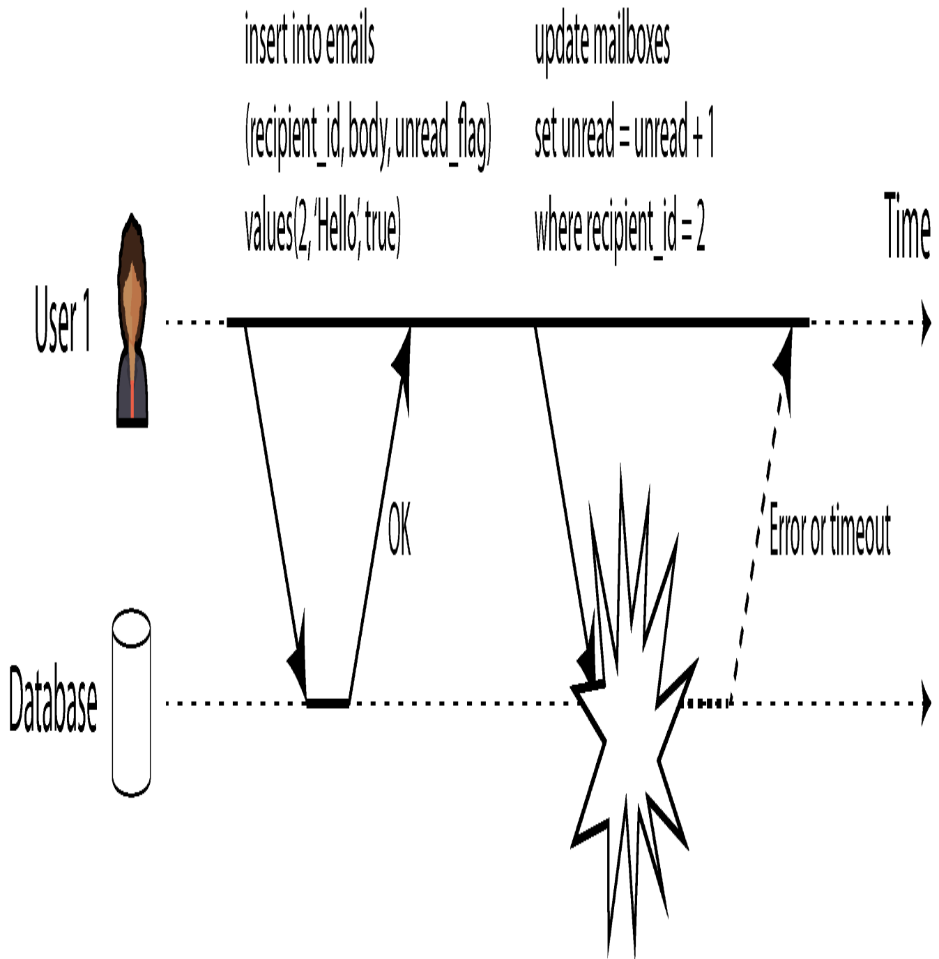
Figure 8-3. Atomicity ensures that if an error occurs, any prior writes from that transaction are undone, to avoid an inconsistent state.
