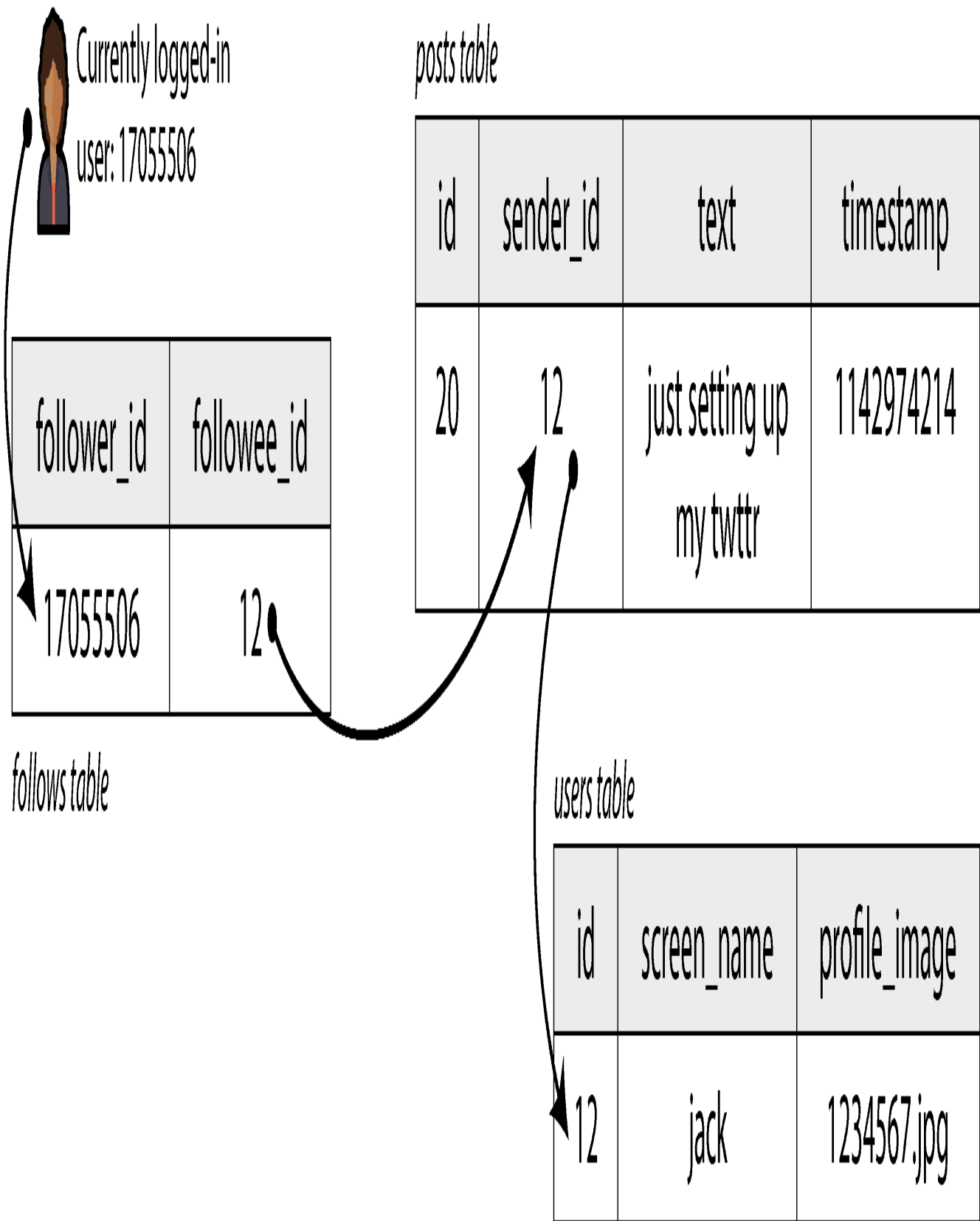
Figure 2-1. A simple relational schema for a social network in which users can follow one another
