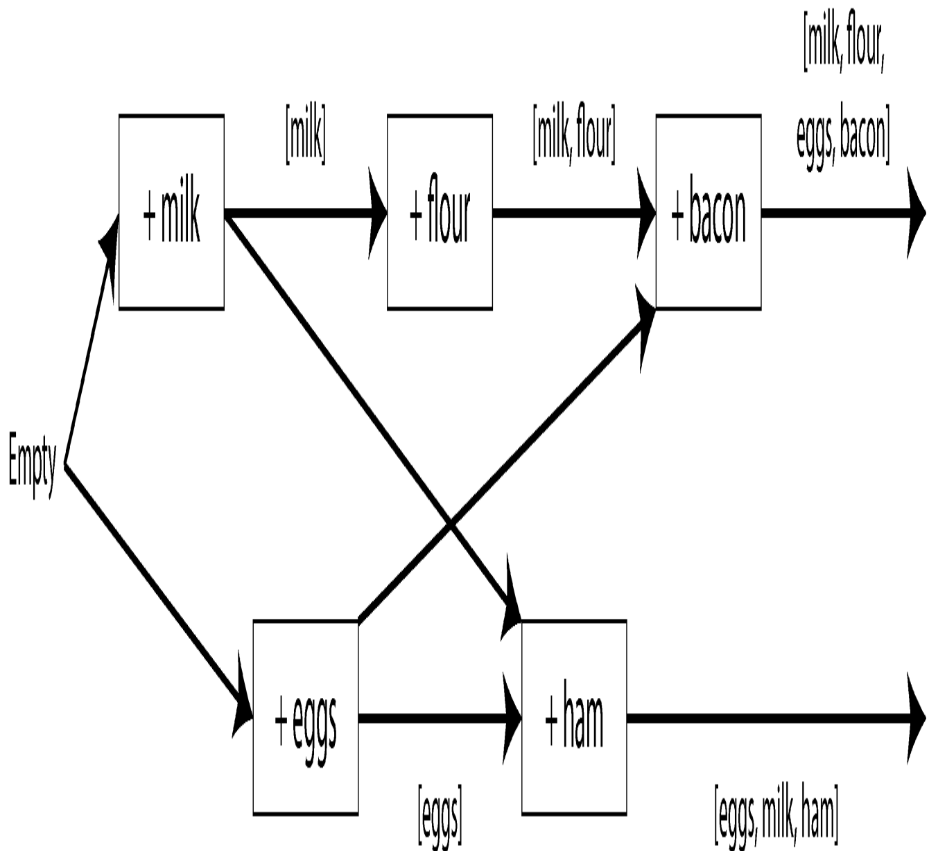
Figure 6-16. A graph of the causal dependencies in Figure 6-15
