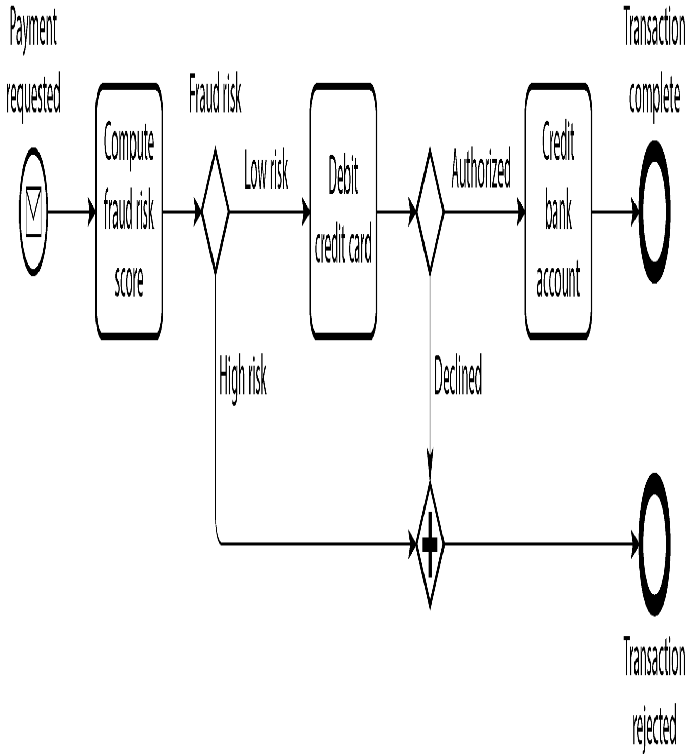
Figure 5-7. A workflow expressed using Business Process Model and Notation (BPMN), a graphical notation
