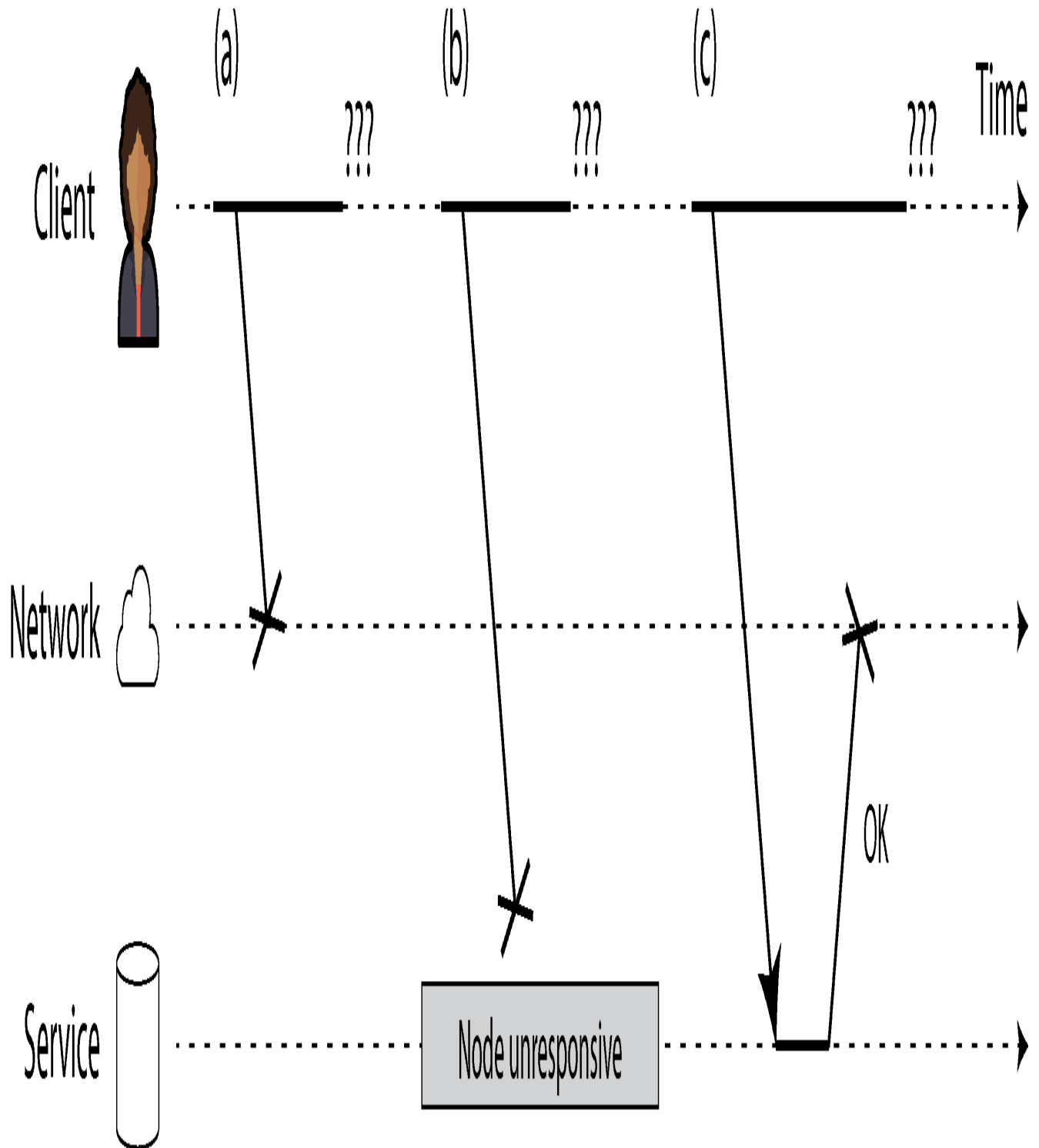
Figure 9-1. If you send a request and don't get a response, it's not possible to distinguish whether (a) the request was lost, (b) the remote node is down, or (c) the response was lost.
