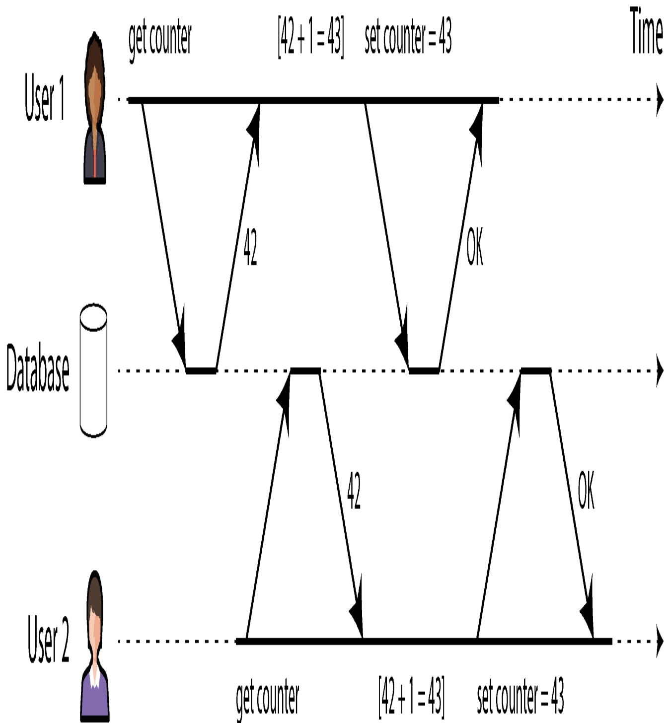
Figure 8-1. A race condition between two clients concurrently incrementing a counter
