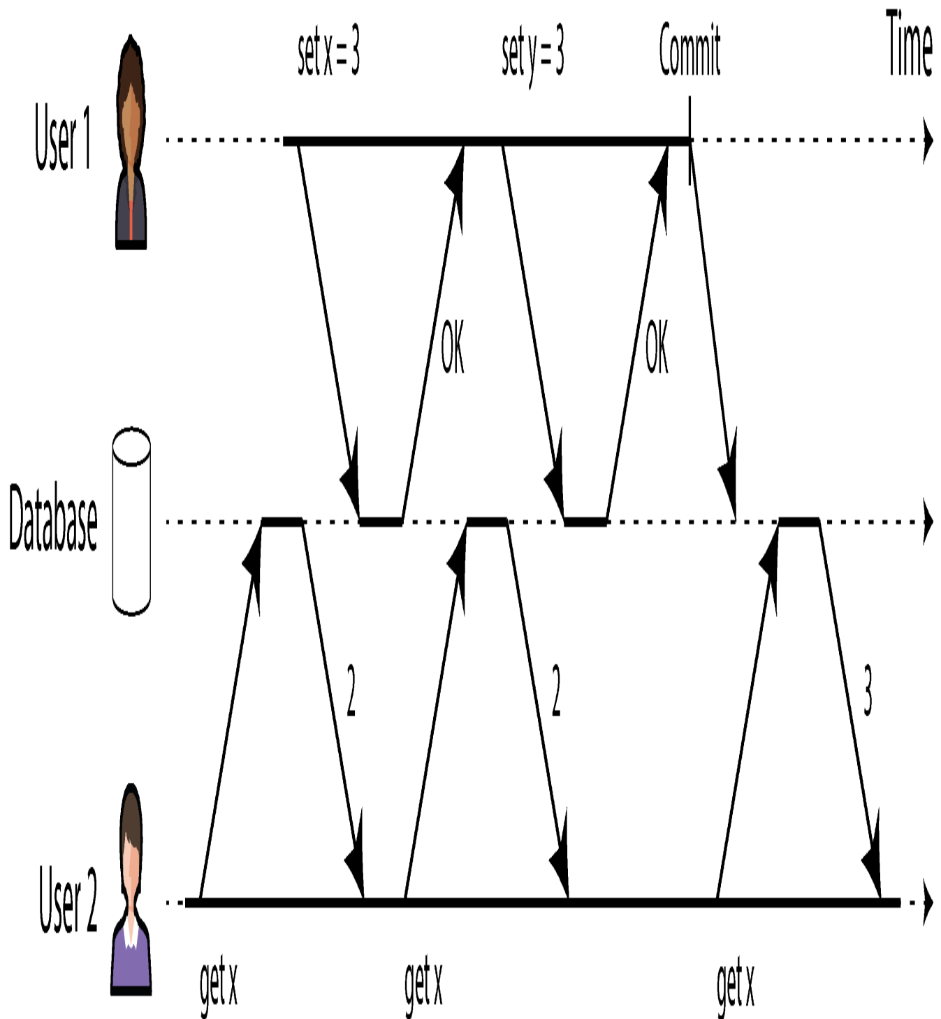
Figure 8-4. No dirty reads: user 2 sees the new value for x only after user 1's transaction has committed
