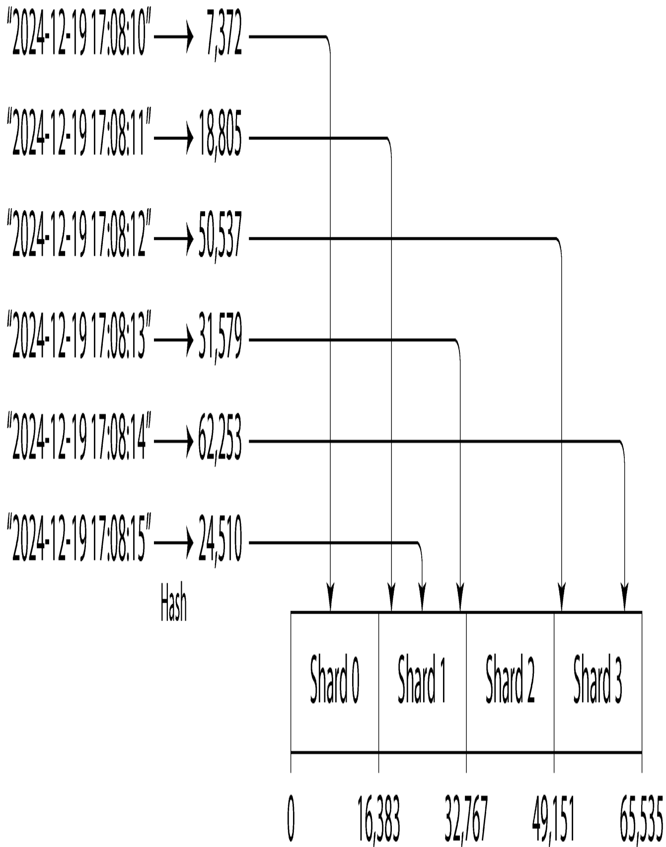
Figure 7-5. Assigning a contiguous range of hash values to each shard
