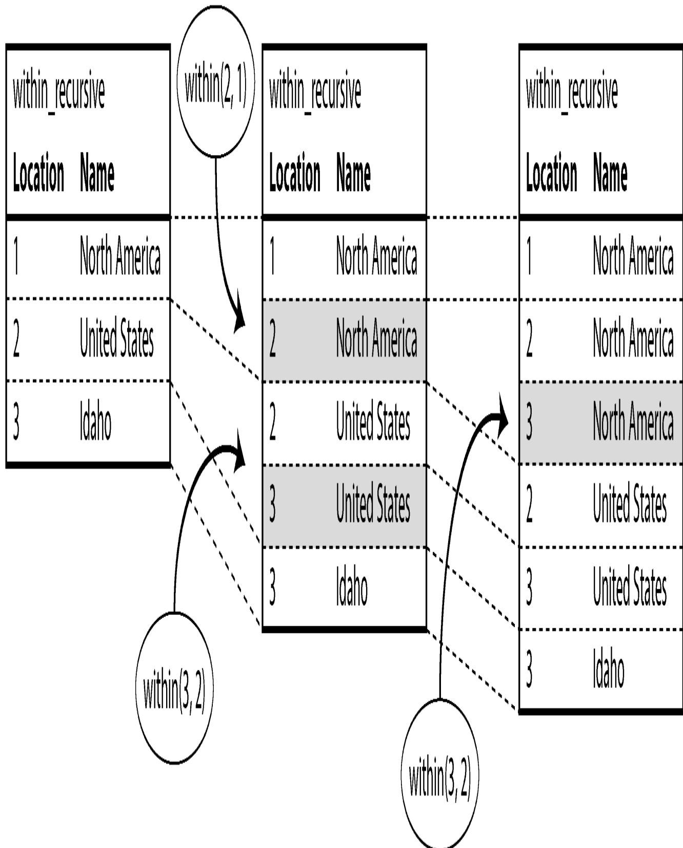
Figure 3-7. Determining that Idaho is in North America, using the Datalog rules from Example 3-12
